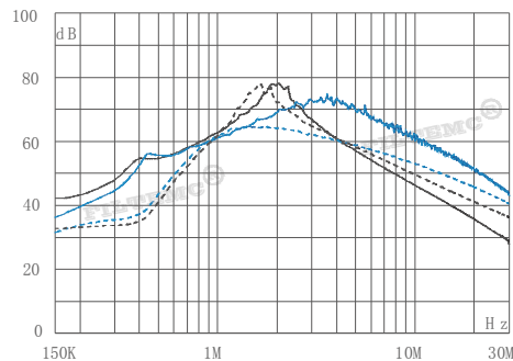
■ FT110PD-0.5 ■ FT110PD-1
