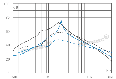
■ FT110PD-3 ■ FT110PD-6
